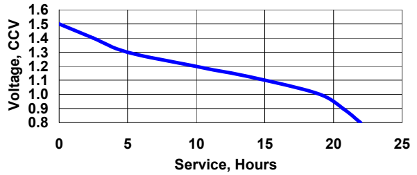
PORTABLE LIGHTING 3.9 ohm - 4 min/hr 8 hr/day
